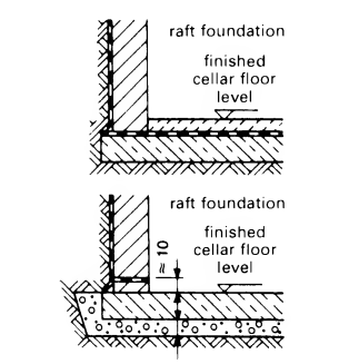
⑩ Damp-proofing and tanking of building with cellar; masonry walls on a raft foundation
